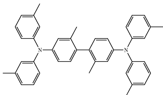
HMTDP
