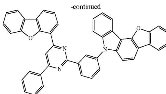
Molecular Weight: 653.73 Compound 814
