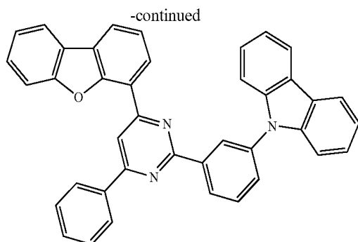
Molecular Weight: 563.65 Compound 813
