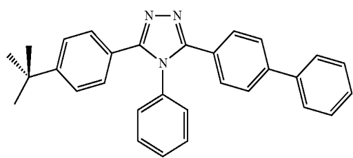
TAZ
